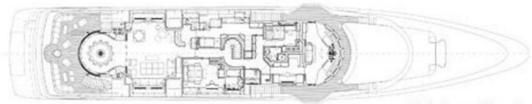
Bridge Deck
